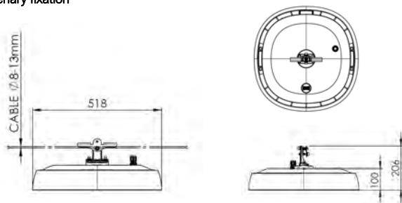
Catenary fixation
